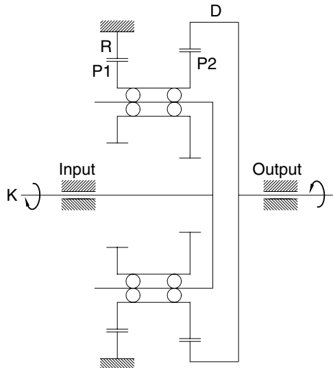
Differential gear mechanism
