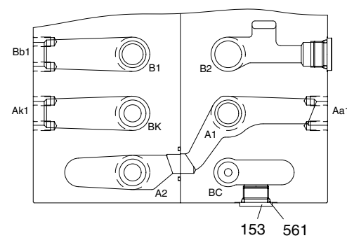
SECTION N-N
