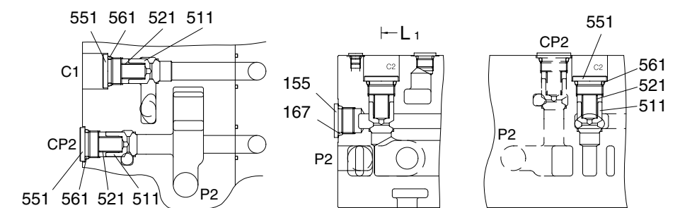
SECTION K-K
