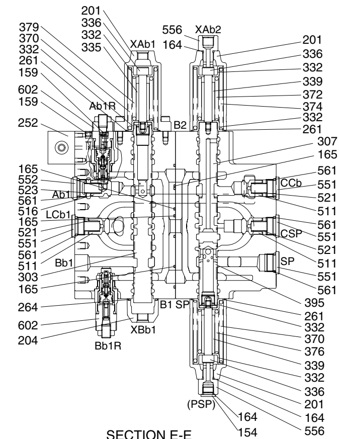
SECTION E-E
