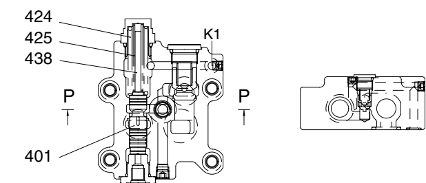
SECTION J-J
