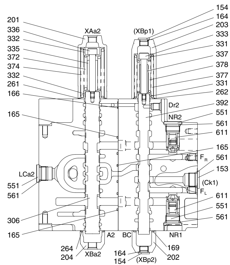
SECTION G-G
