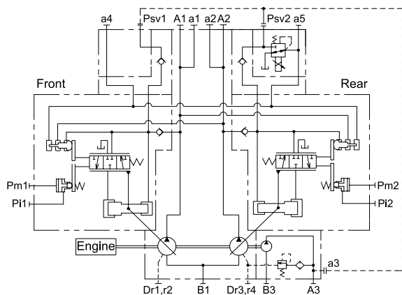
Hydraulic circuit
