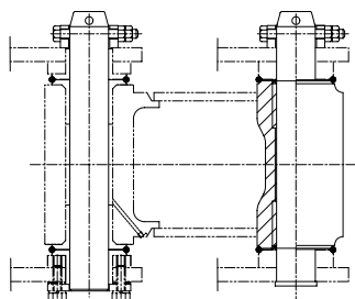
SECTION A
