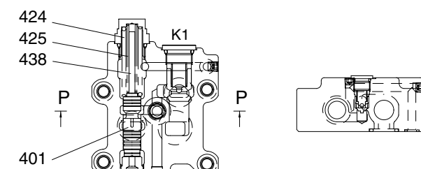
SECTION J-J
