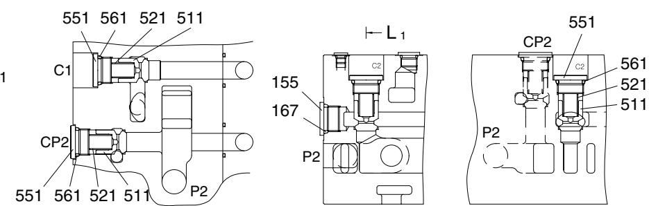
SECTION K-K
