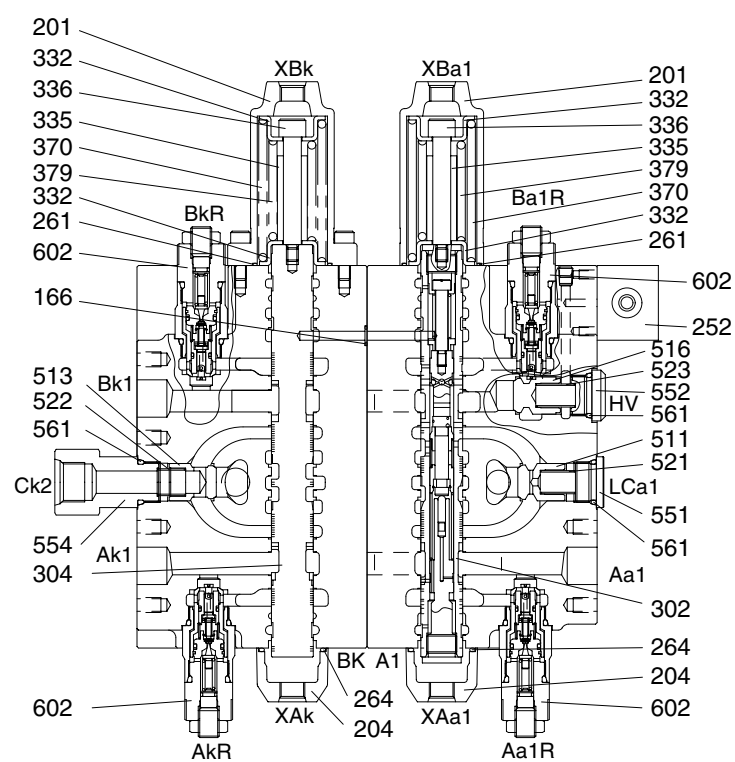
SECTION C-C
