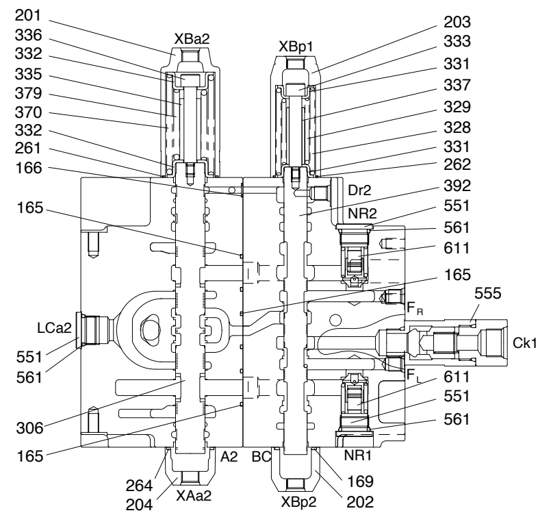
SECTION G-G
