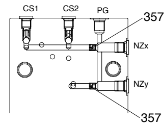
SECTION H-H
