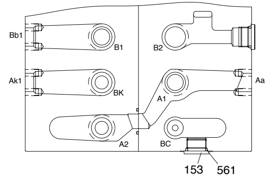
SECTION N-N
