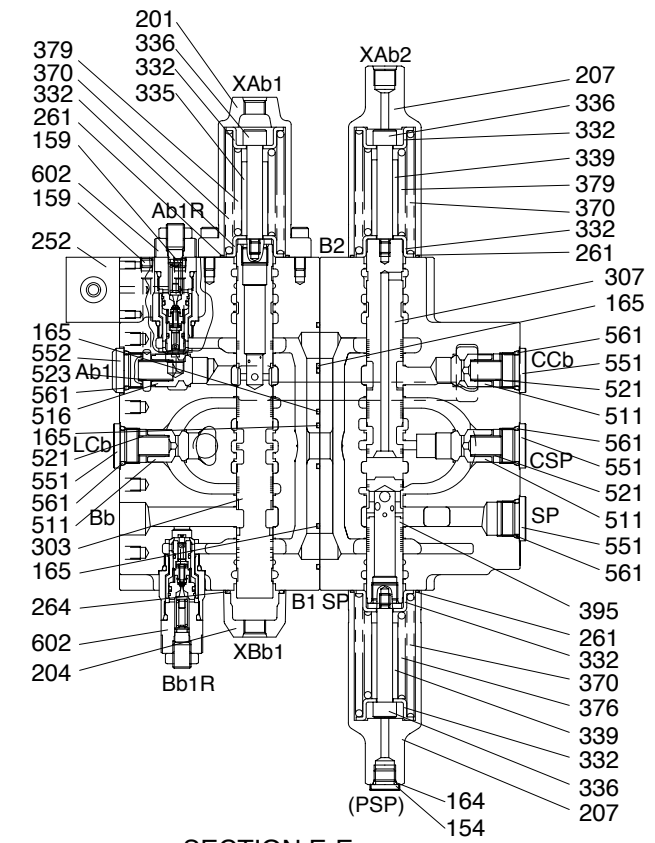
SECTION E-E
