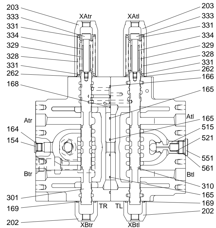
SECTION C-C
