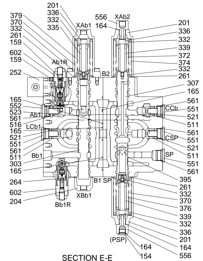
SECTION E-E
