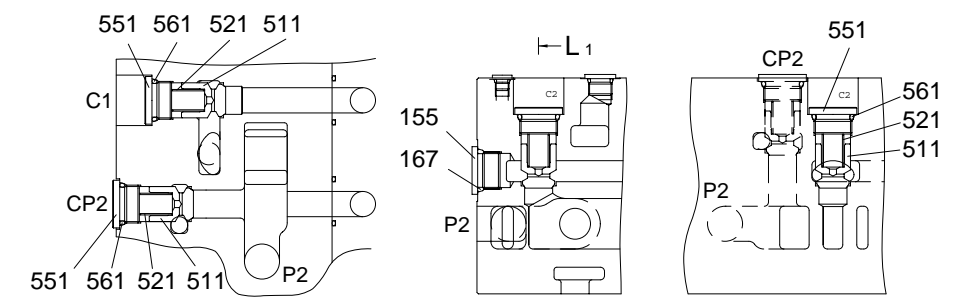
SECTION K-K
