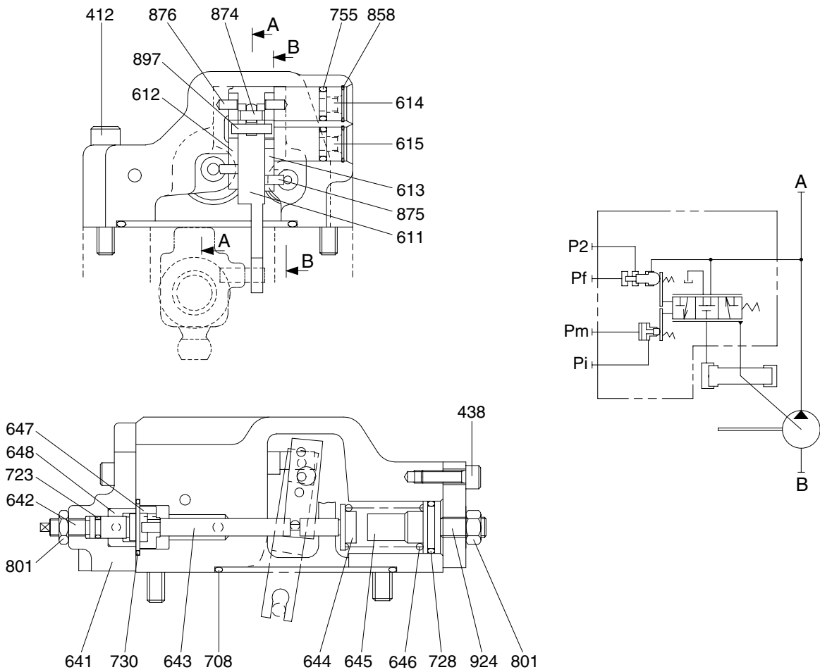
SECTION B-B
