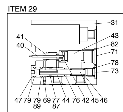
LOCK VALVE - A KIT(BOOM & ARM)
