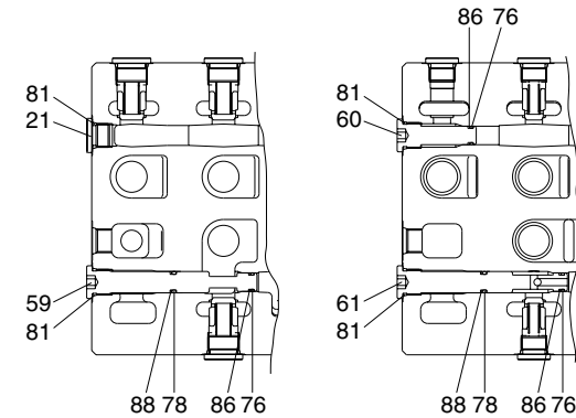
G - G(OPTION-C & NEGATIVE CONTROL)
