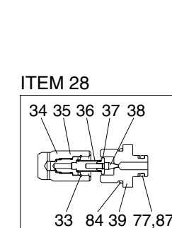
LOCK VALVE - B KIT (BOOM & ARM)
