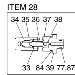
LOCK VALVE - B KIT (BOOM & ARM)
