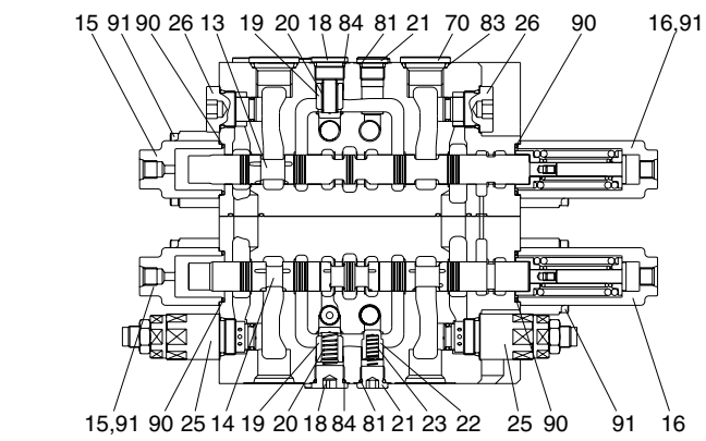
F - F (OPTION-B & BUCKET)
