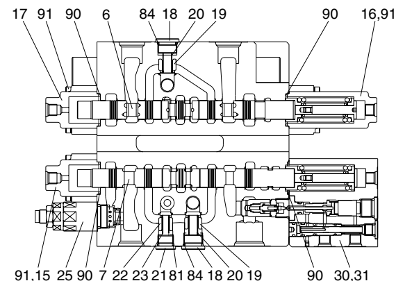
C - C (SWING & BOOM 1)
