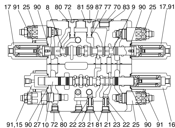
D - D (SWING PRIORITY & BOOM 2 & ARM 2)
