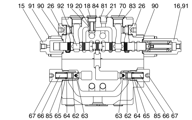
G - G (OPTION-C & NEGATIVE CONTROL)
