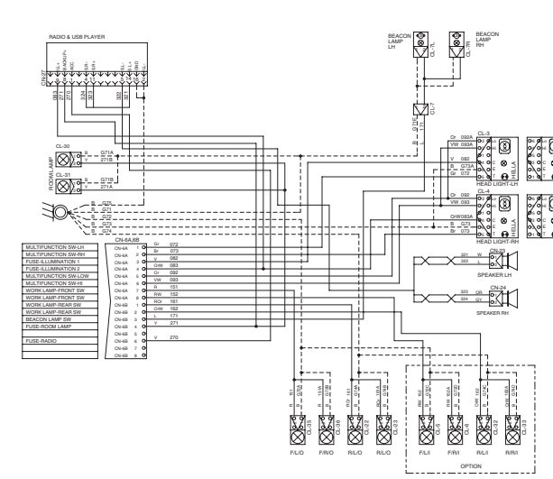
H930S/H940S CAB TYPE
