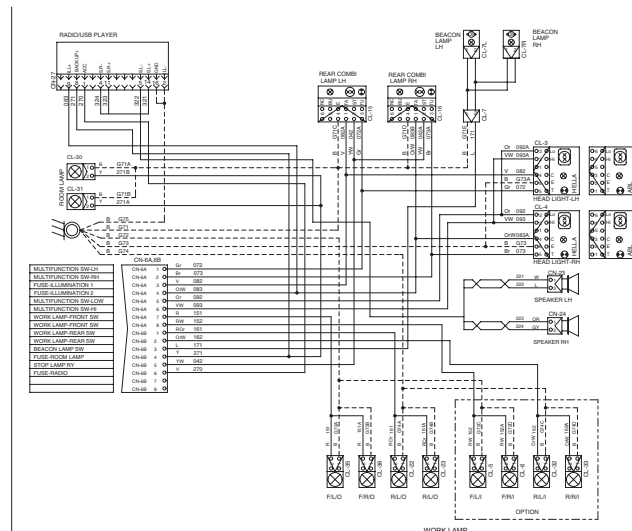
H930C/H940C CAB TYPE
