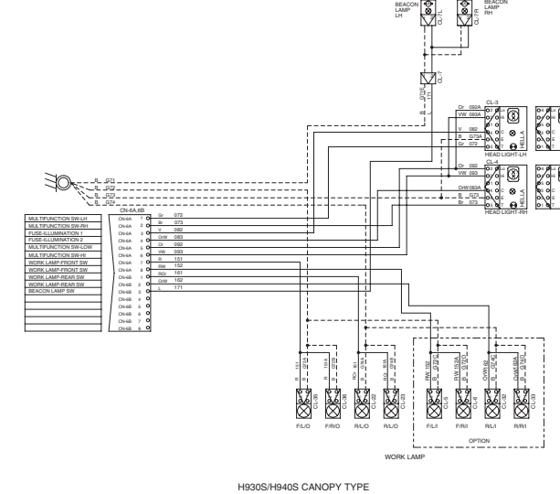
H930S/H940S CANOPY TYPE
