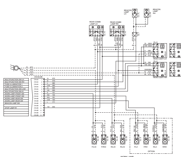
H930C/H940C CANOPY TYPE
